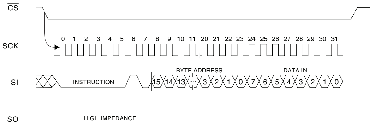
Figure 4-7. WRITE Timing
