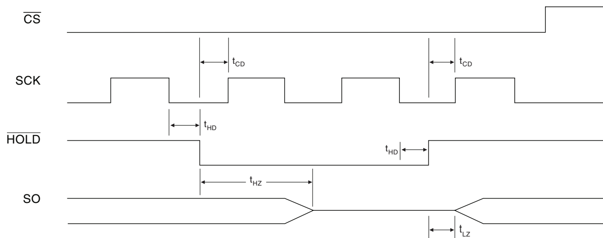
Figure 4-8. \overline{\text{HOLD}} Timing
