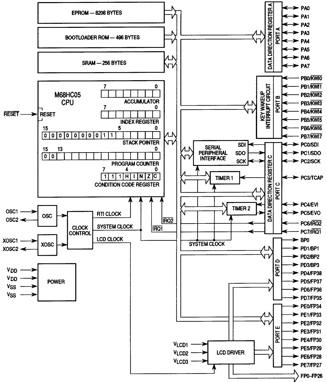
MCU Structure
