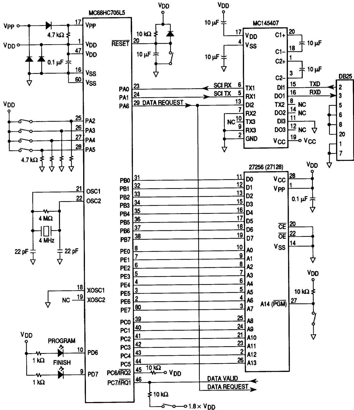
Bootloader Circuit
