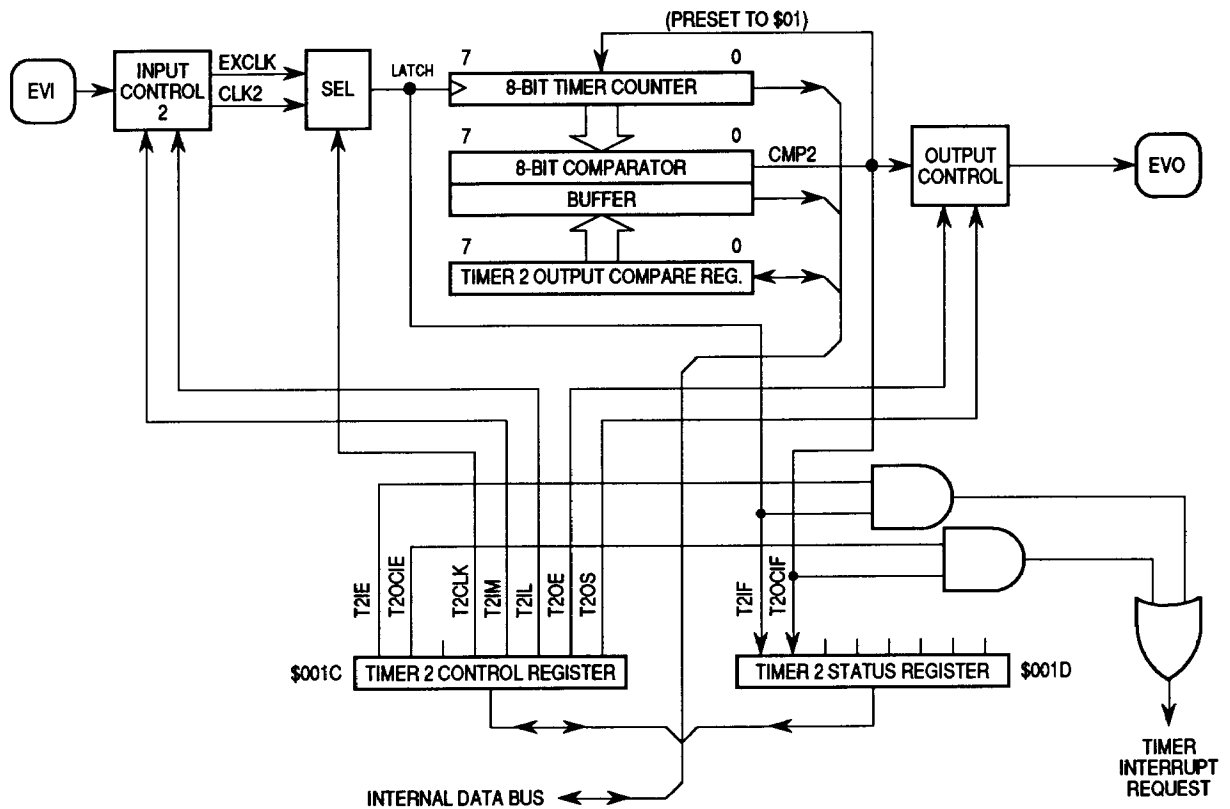
Timer 2
