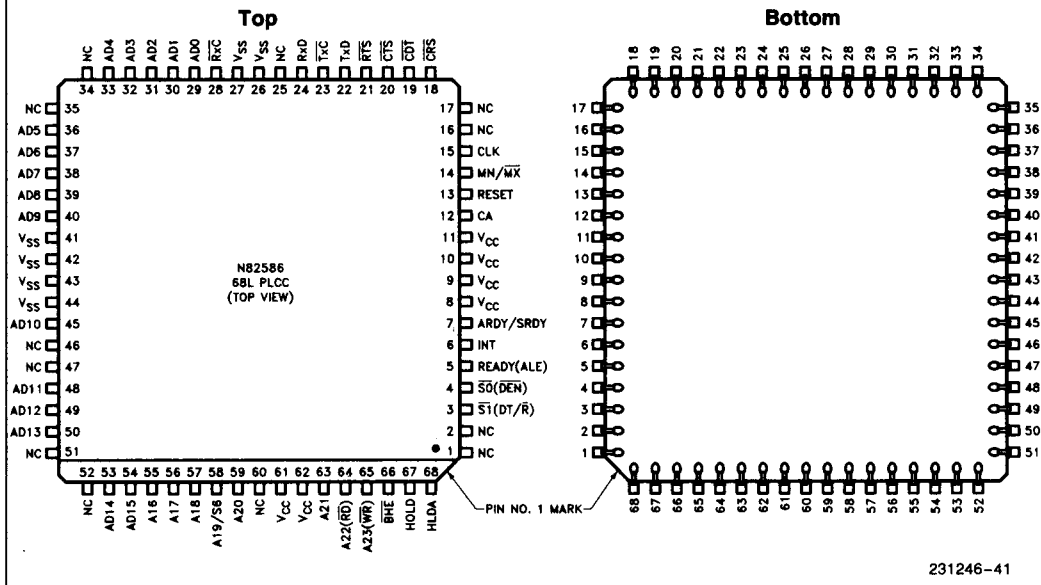
Figure 2. 82586 Pinout Diagrams
