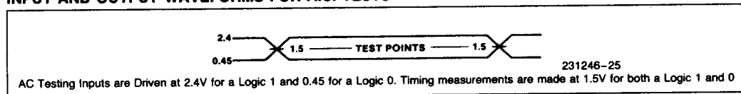
Figure 24. TTL Input/Output Voltage Levels for Timing Measurements
