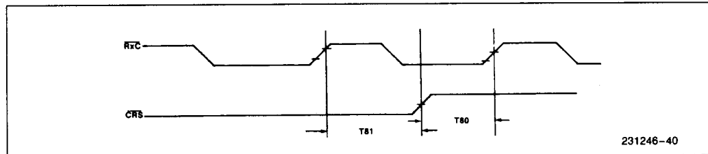
Figure 38. CRS Timing Relative to \overline{RxC}
