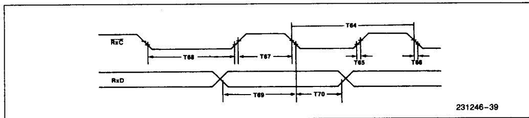
Figure 37. RXD Timing Relative to \overline{RxC}
