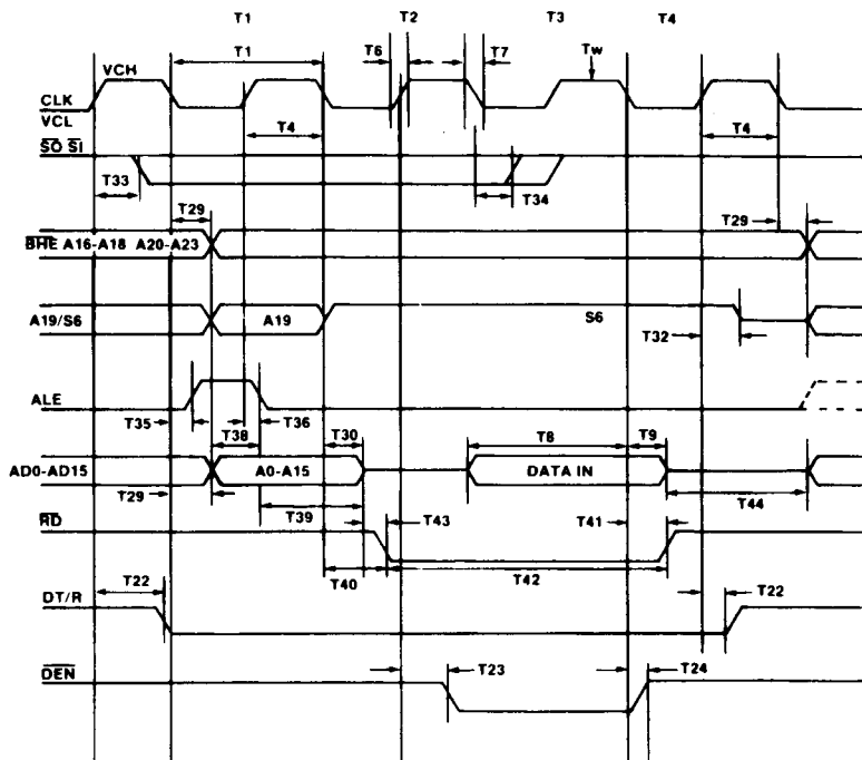
Figure 31. Read Cycle Timing
