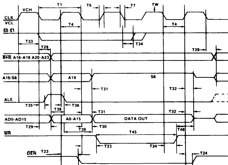
Figure 32. Write Cycle Timing
