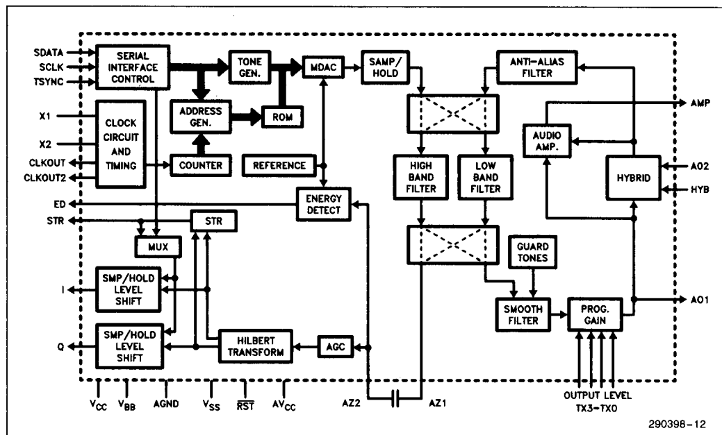
Figure 9. 89027 Block Diagram
