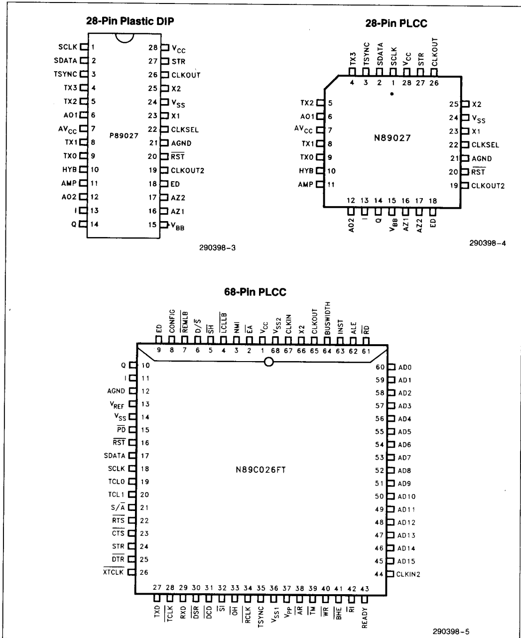
Figure 3. Device Packages
