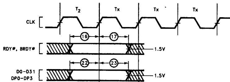
Figure 13.3. Input Setup and Hold Timing
