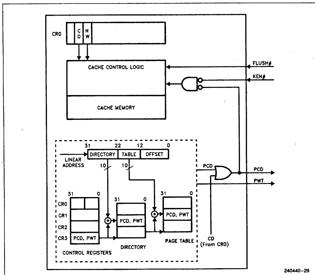
Figure 5.3. Page Cacheability
