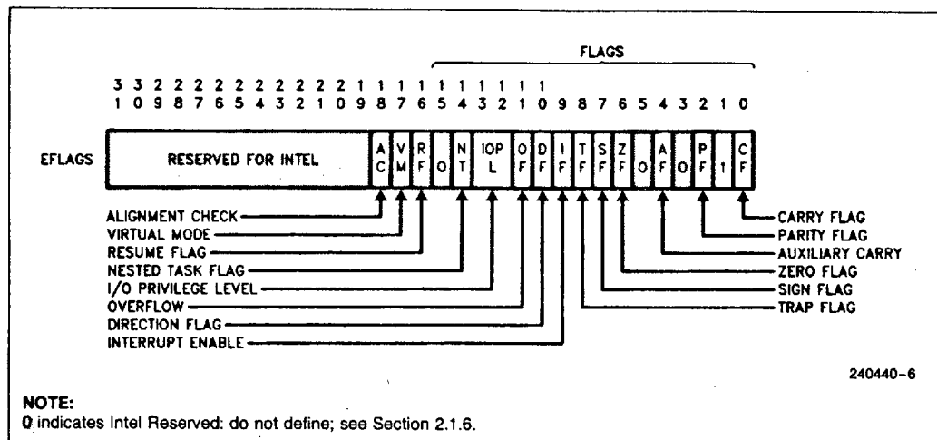
Figure 2.2. Flags Register
