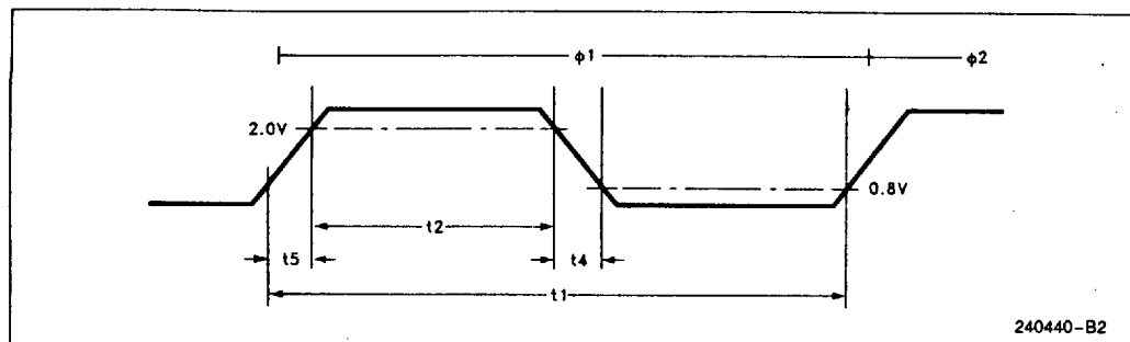
Figure 15.8. CLK2 Waveform
