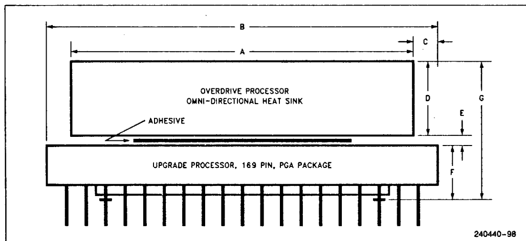
Figure 12.2. Intel OverDrive™ Processor, 169-Pin, PGA Package with Heat Sink Attached
