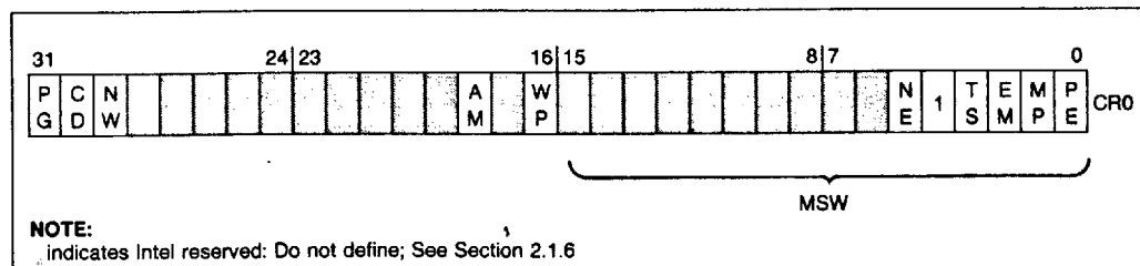
Figure 2.5. Control Register 0
