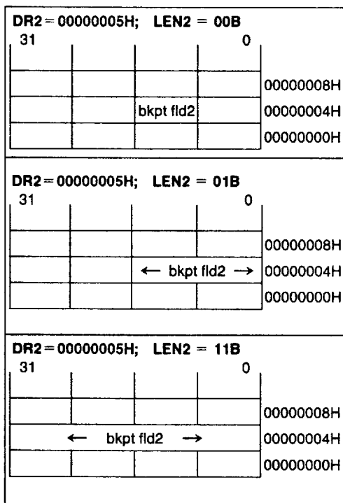
Figure 9.1. Debug Registers
