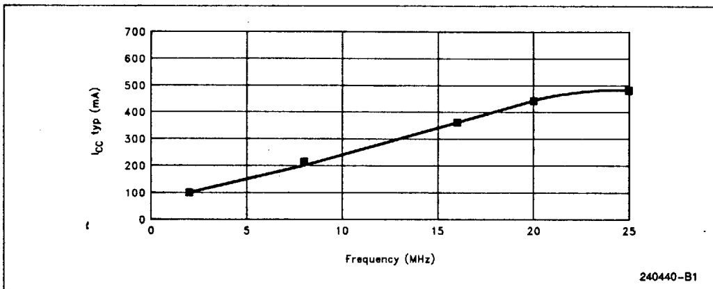
Figure 15.7. Frequency vs I_{CC}(\text{typ}) (PQFP Version)
