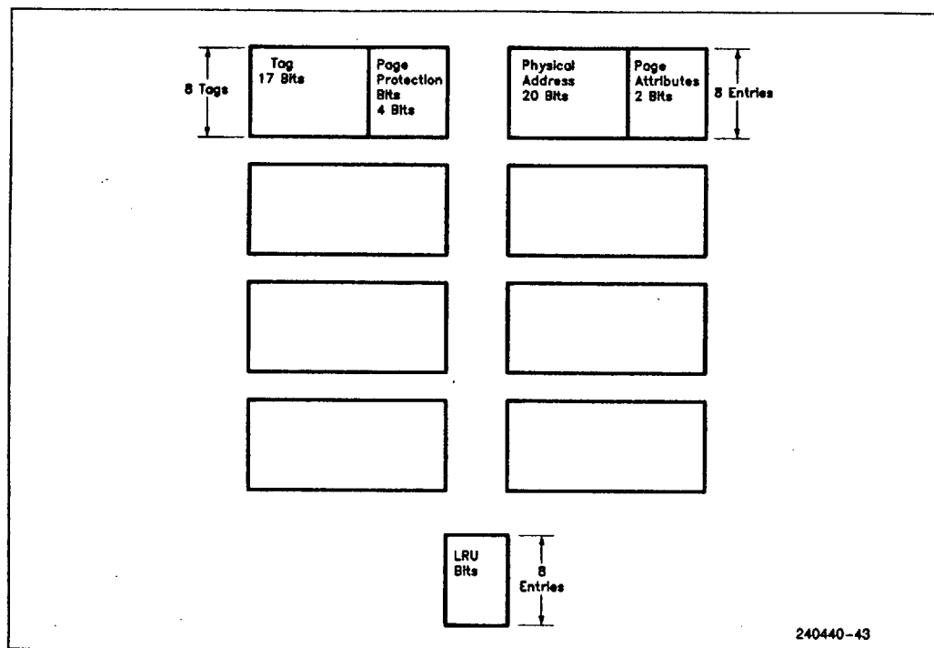
Figure 8.3. TLB Organization
