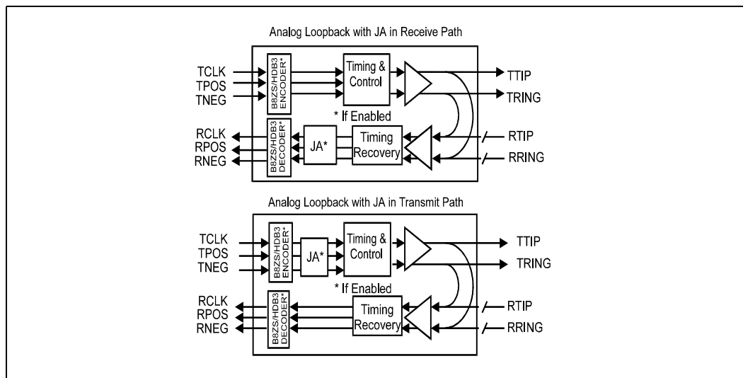
Figure 7. Analog Loopback
