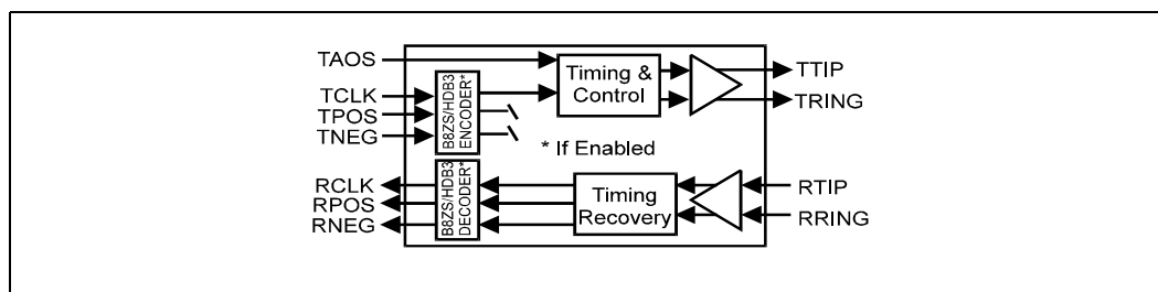
Figure 10. TAOS Data Path
