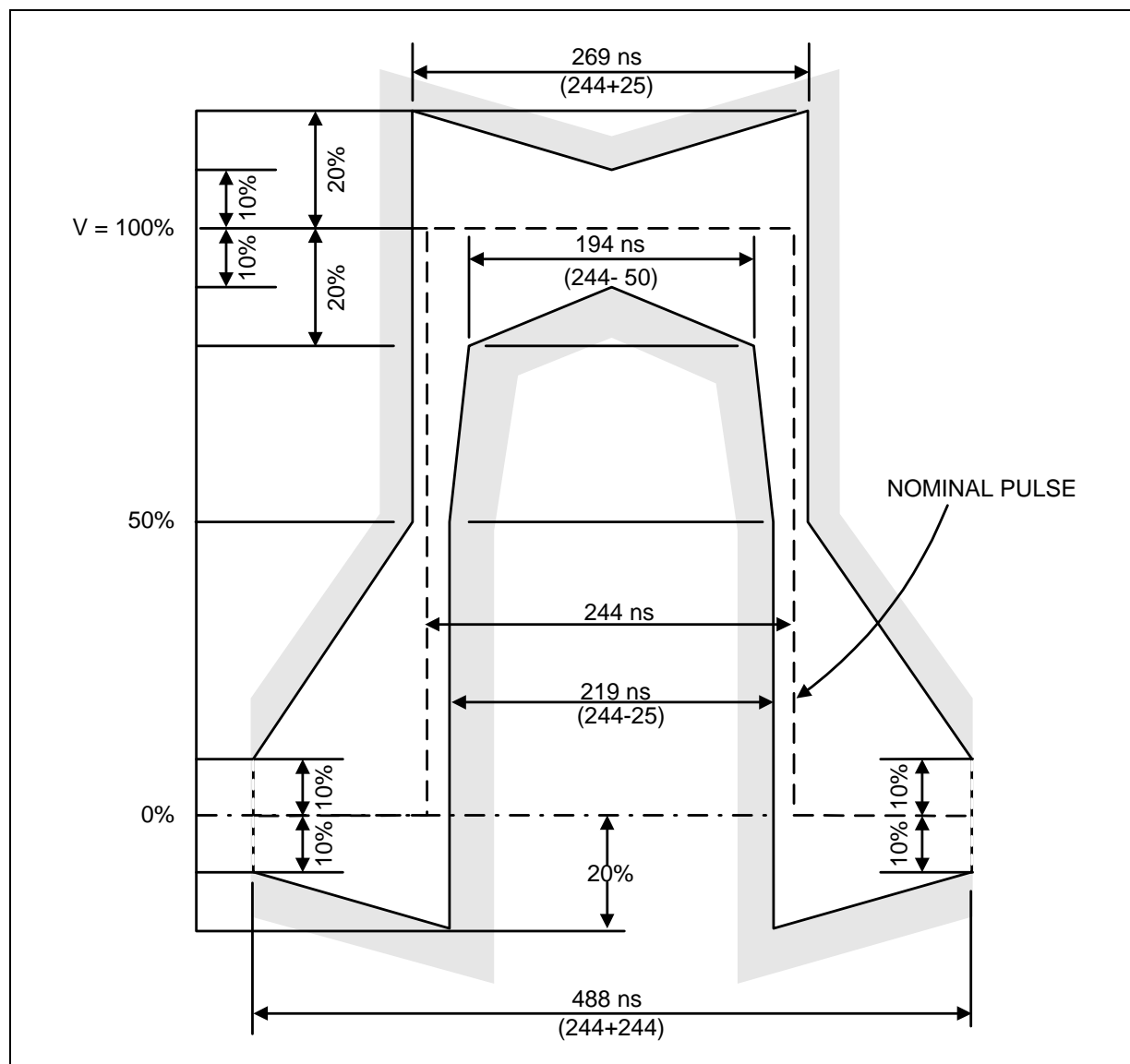
Figure 14. 2.048 MHz E1 Pulse (See Table 29)
