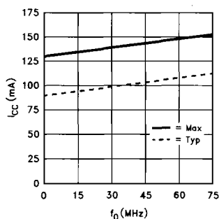
IPLD22V10 I_{CC} vs Frequency
