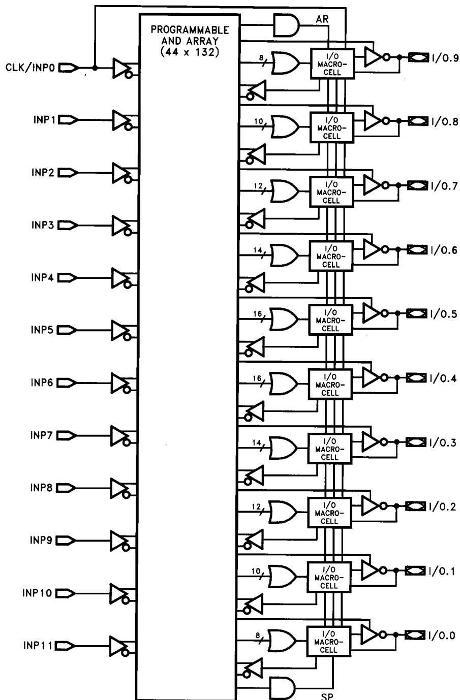
Figure 2. IPLD22V10 Global Architecture
