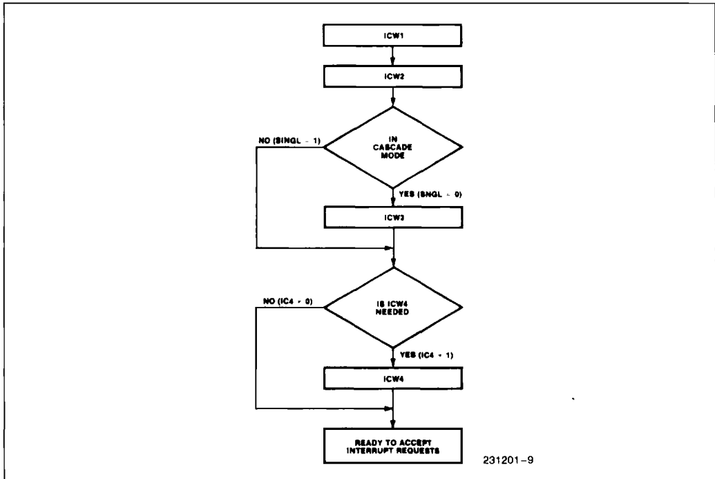
Figure 6. Initialization Sequence
