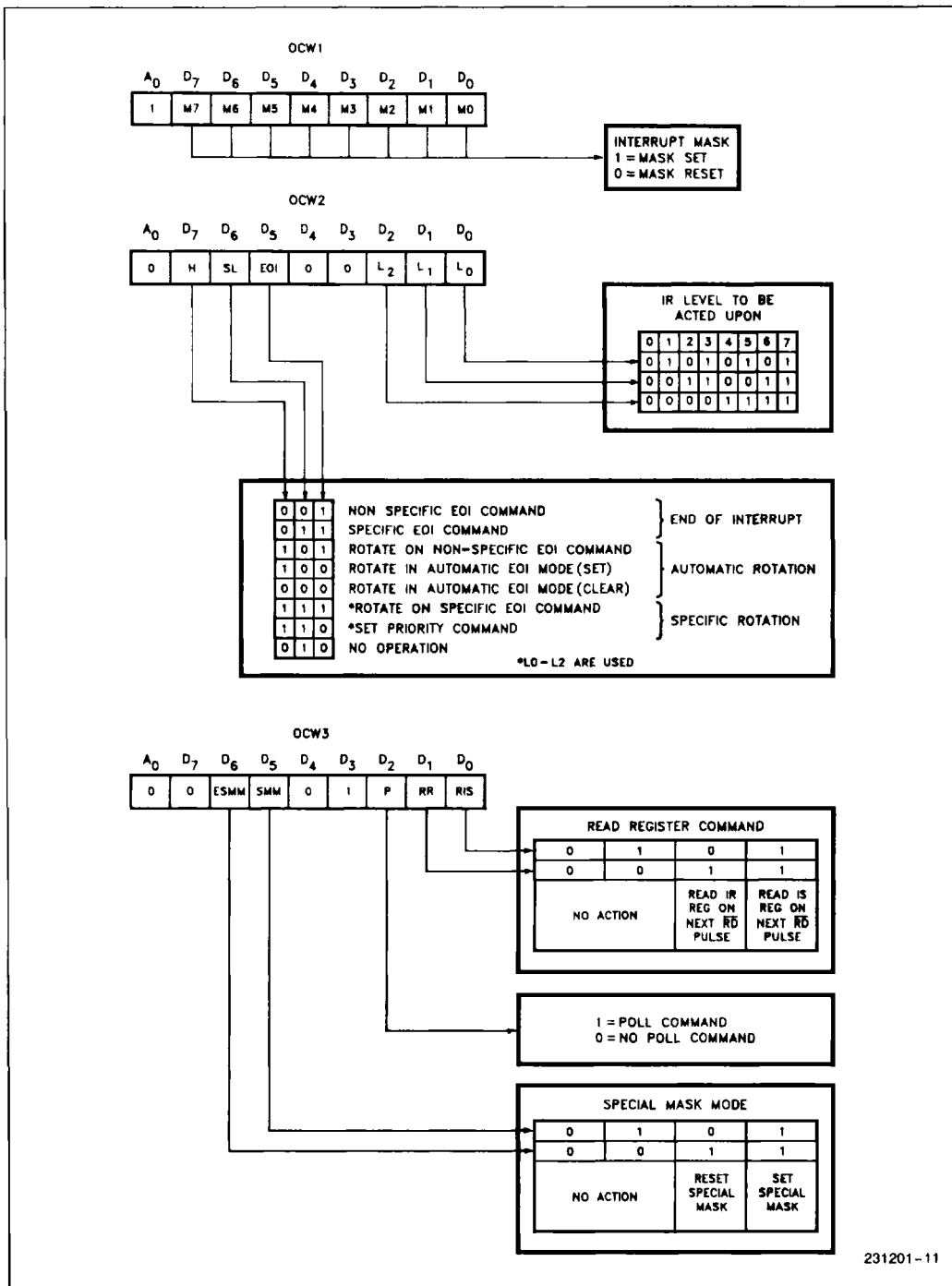
Figure 8. Operation Command Word Format
