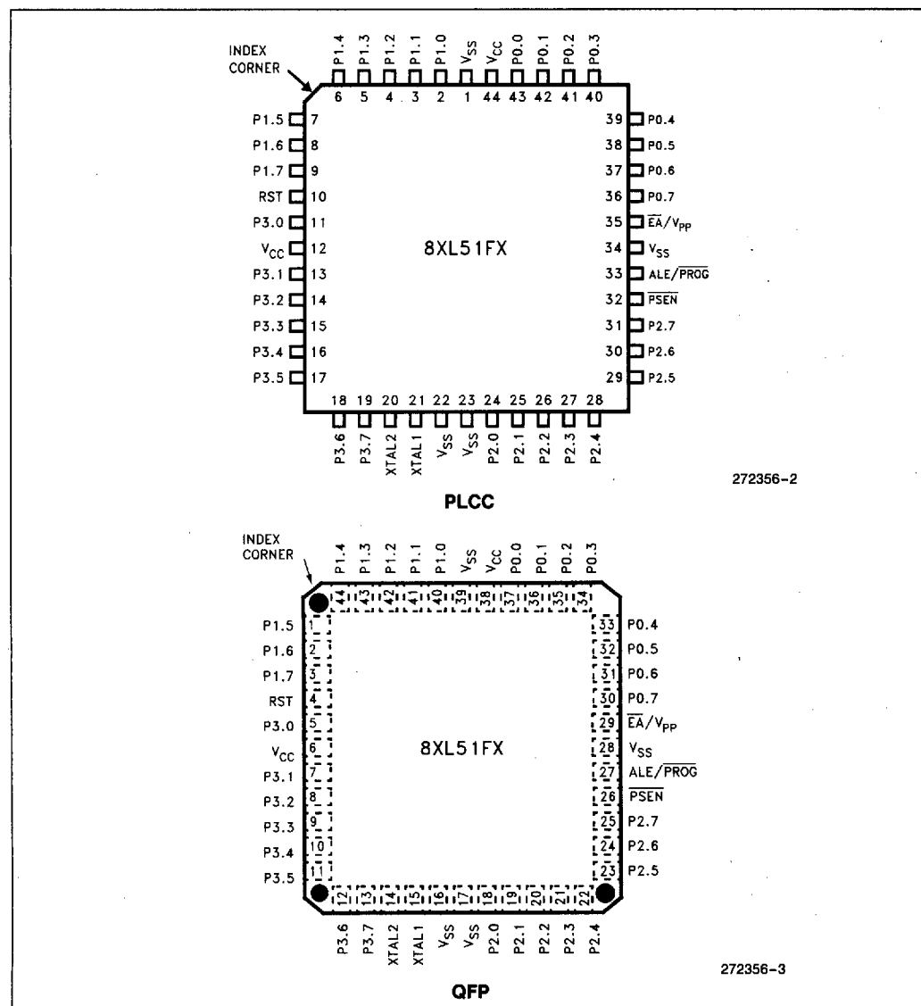
Figure 2. Pin Connections
