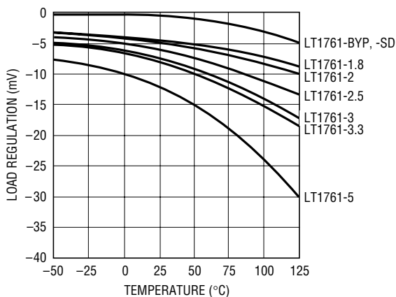
Load Regulation ΔI L = 1mA to 50mA
