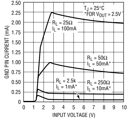
LT1761-2.5 GND Pin Current
