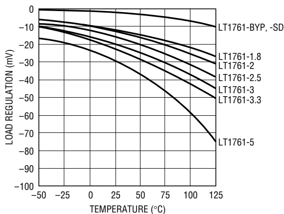
Load Regulation ΔI L = 1mA to 100mA
