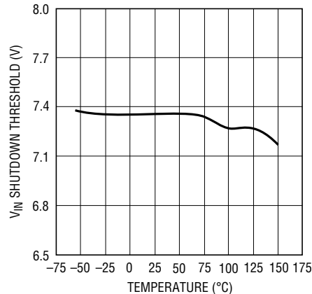
V_{IN} Shutdown Threshold vs Temperature
