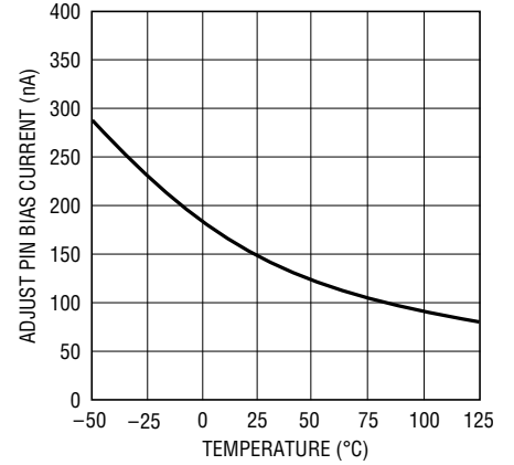
LT1121 Adjust Pin Bias Current
