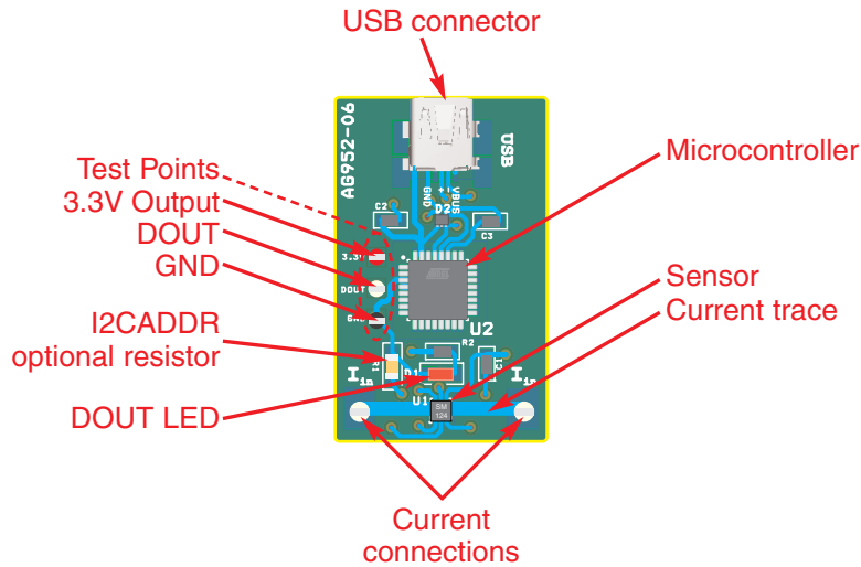
Figure 13. AG952-07E: Smart Current Sensor Evaluation Kit board 1" x 1.625" (25 mm x 41 mm) (actual size)
