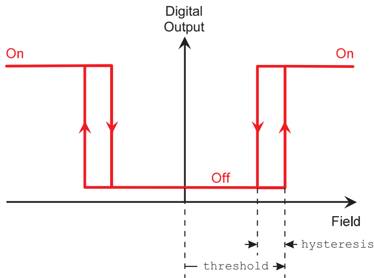
Figure 8. Digital Output parameters.
