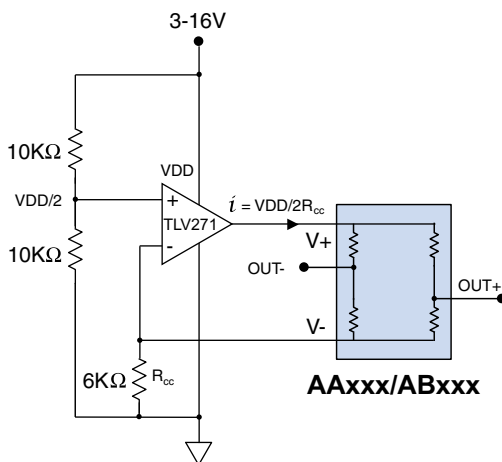
Figure 11. Constant-current supply.
