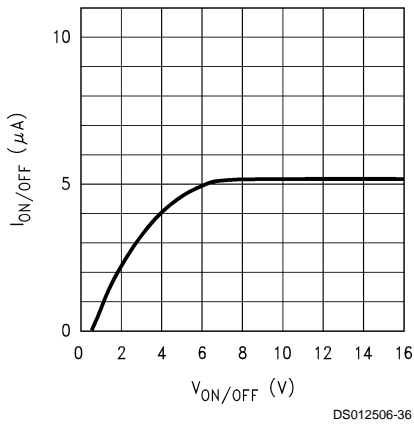
ON/OFF Pin Current vs V_{ON/OFF}
