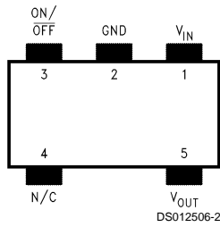
5-Lead Small Outline Package (M5)
