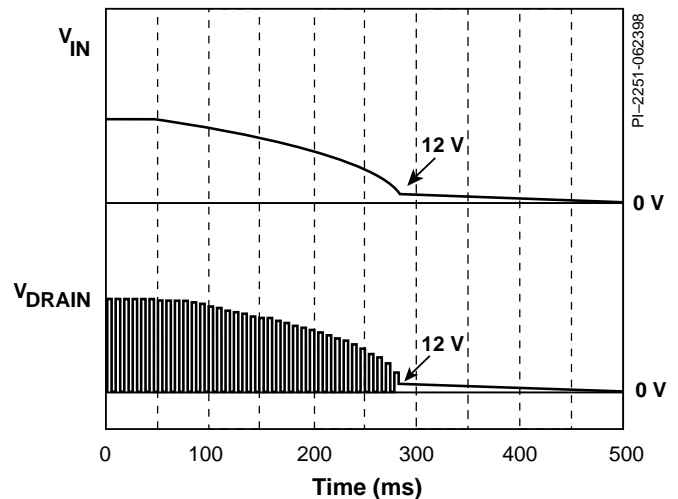
Figure 8. TinySwitch Power Down Timing Diagram.
