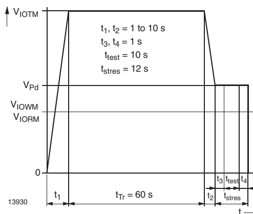
Figure 2. Test pulse diagram for sample test according to DIN EN 60747-5-2(VDE0884)/ DIN EN 60747-5; IEC60747
