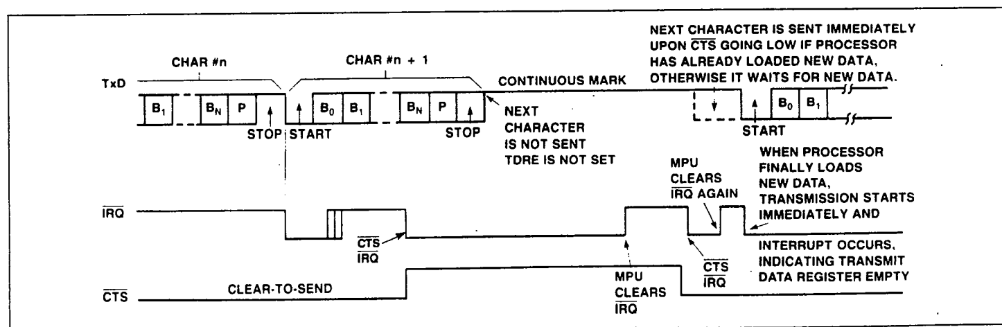
Figure 10. Effects of \overline{\text{CTS}} on Transmitter
