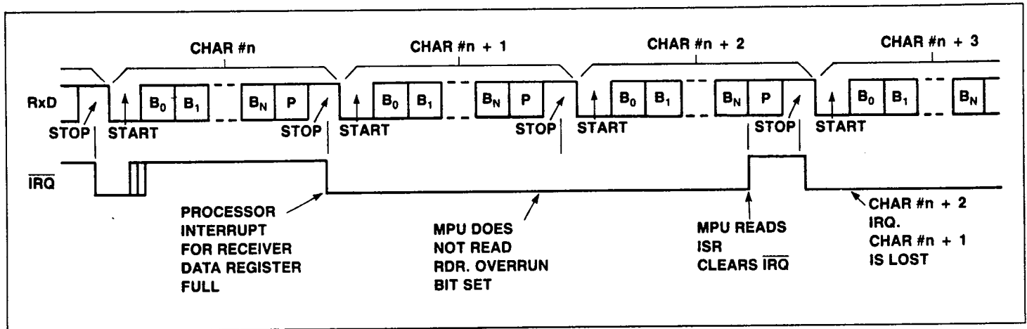
Figure 13. Effects of Overrun on Receiver
