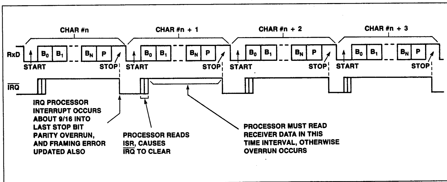
Figure 12. Continuous Data Receive
