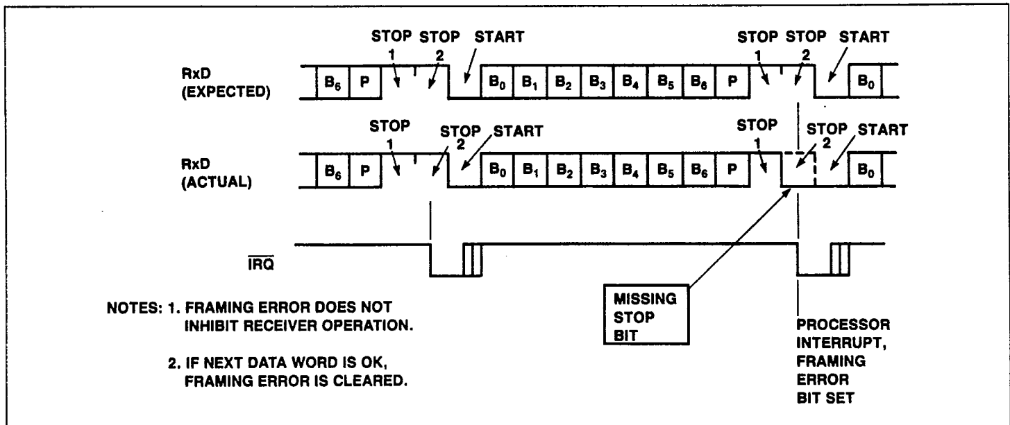
Figure 15. Framing Error
