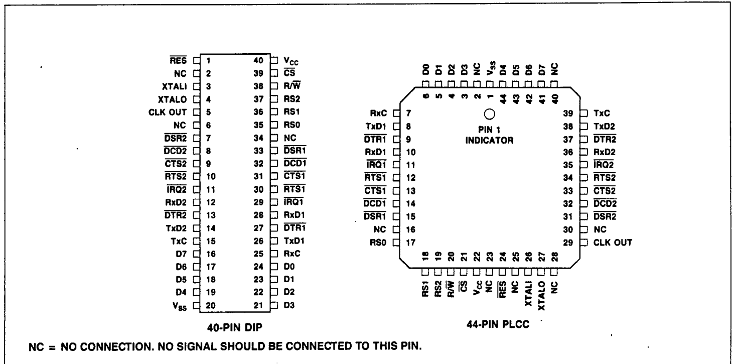
Figure 1. R65C52 Pin Assignments
