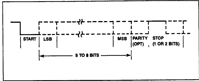
Figure 4. Asynchronous Frame Format
