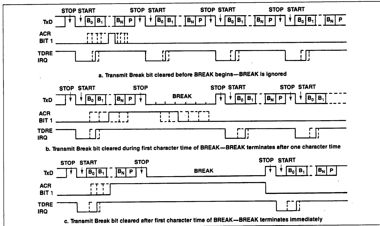
Figure 9. Transmit BREAK
