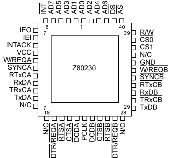
Z80230 PLCC Pin Assignments
